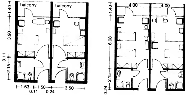
③ One-bed nursing rooms
